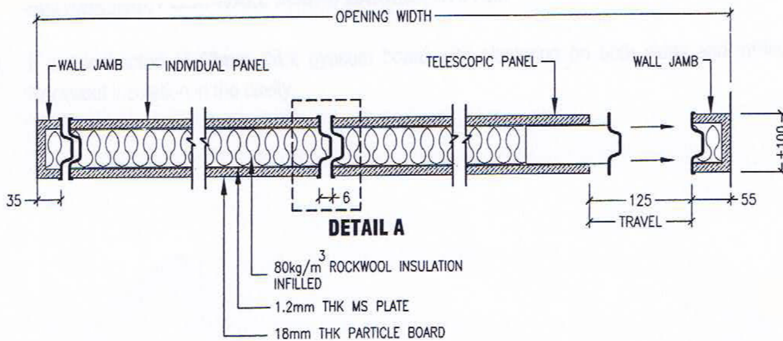
HORIZONTAL SECTION
