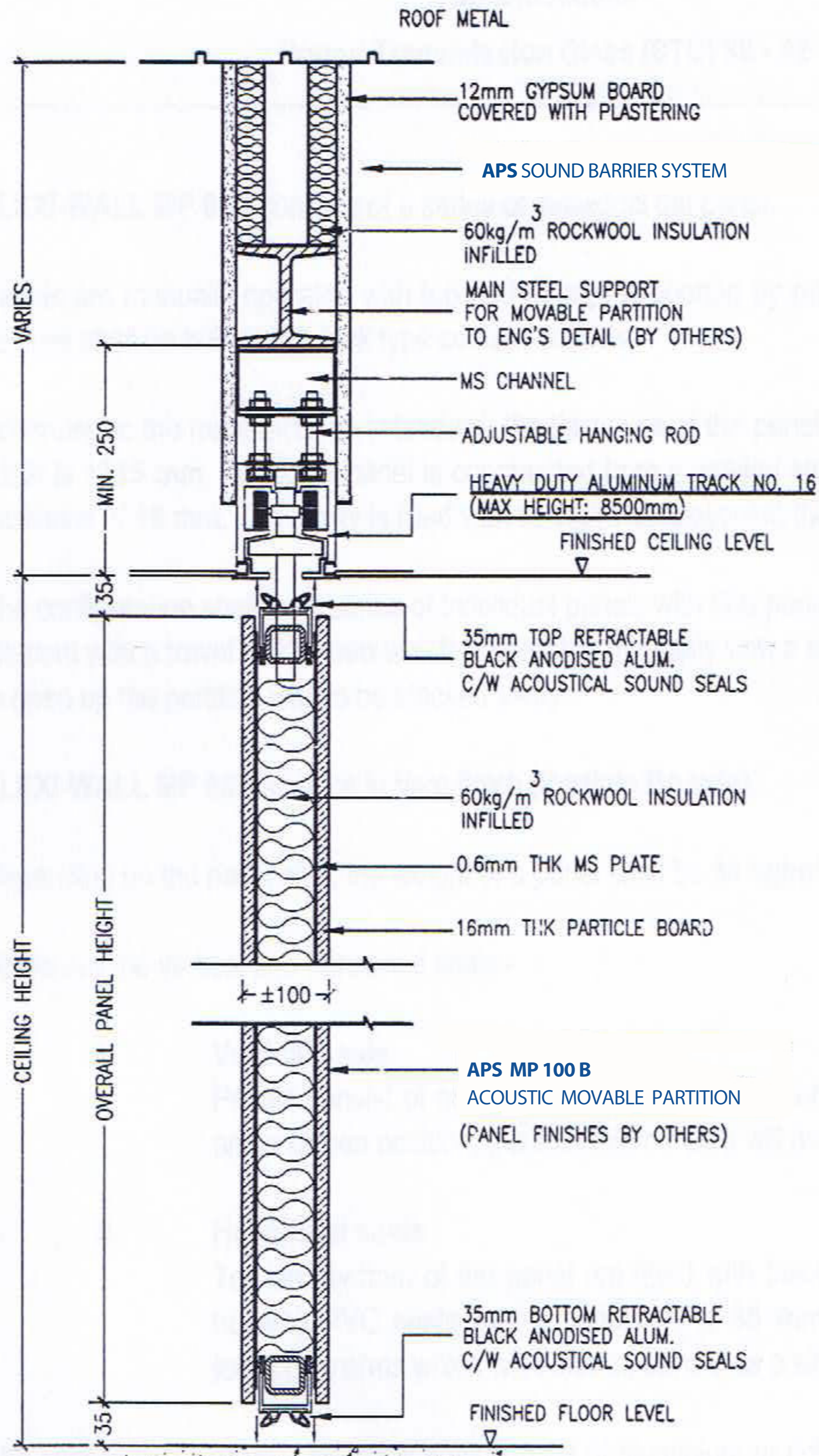
VERTICAL SECTION
