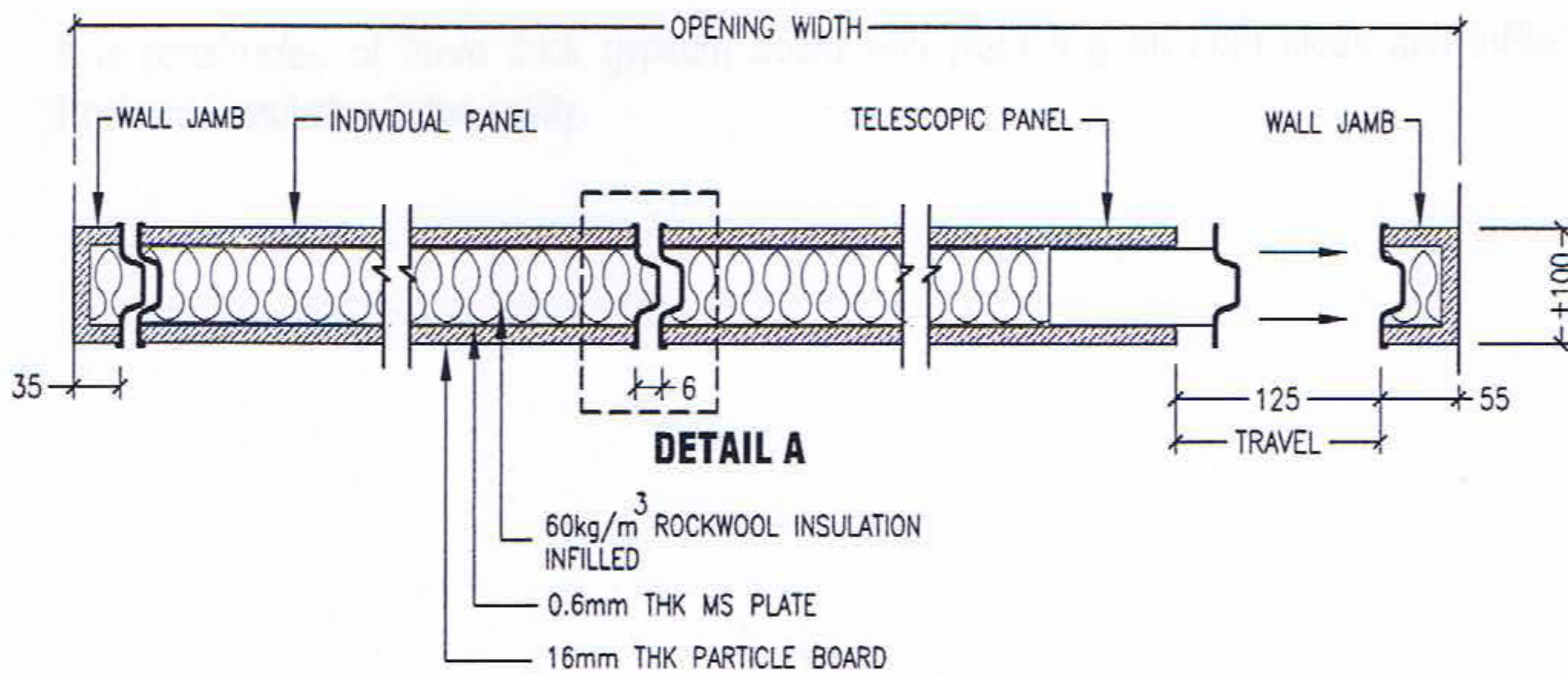
HORIZONTAL SECTION
