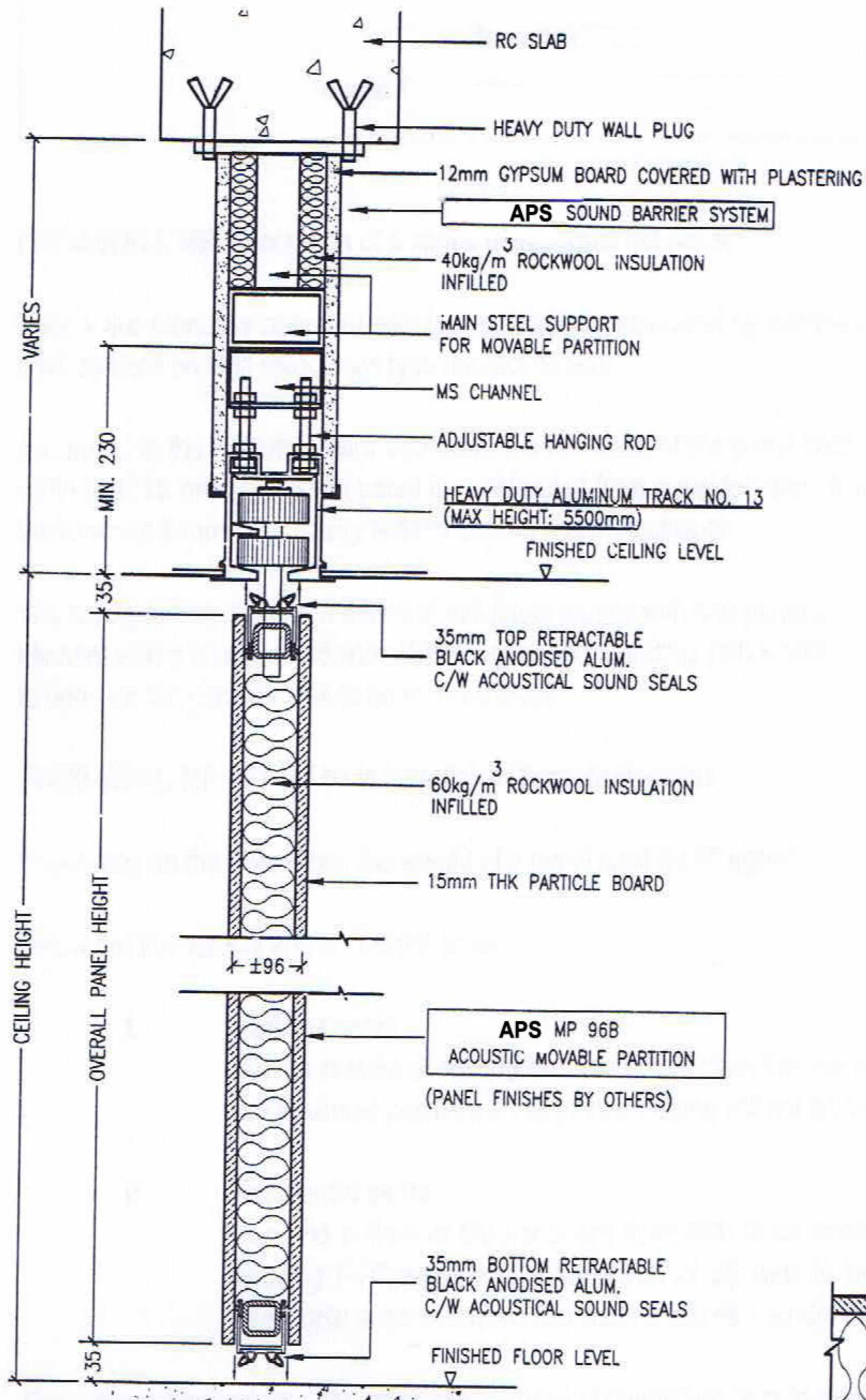
VERTICAL SECTION
