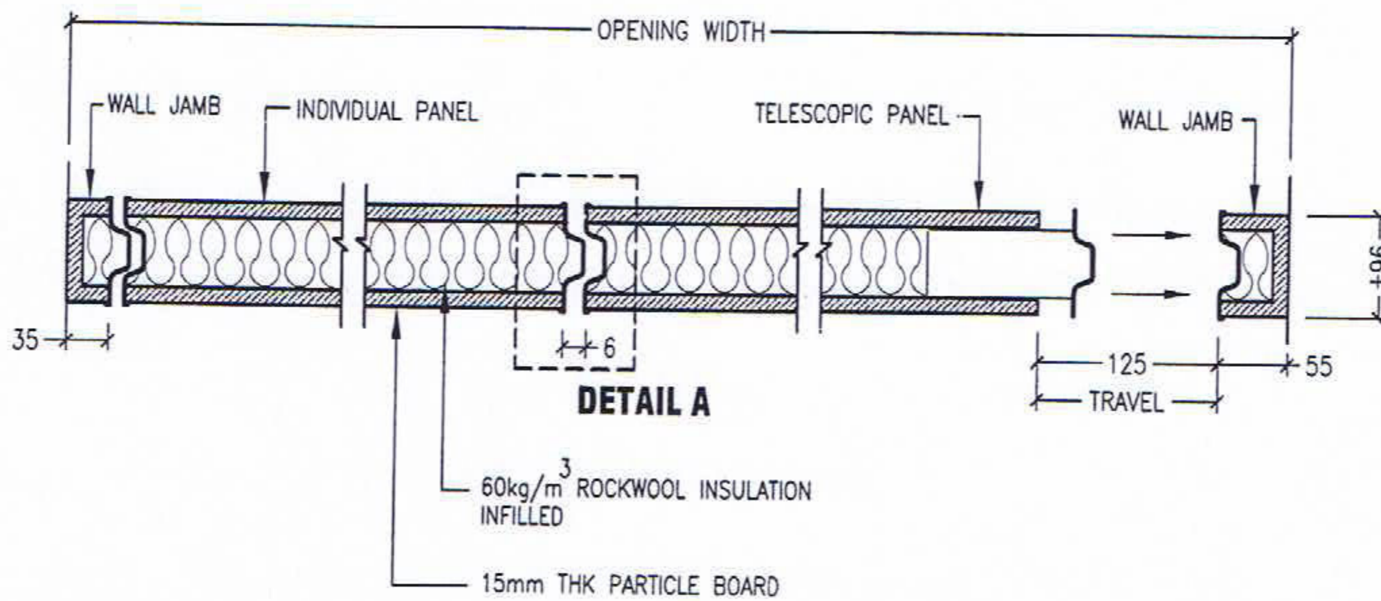
HORIZONTAL SECTION
