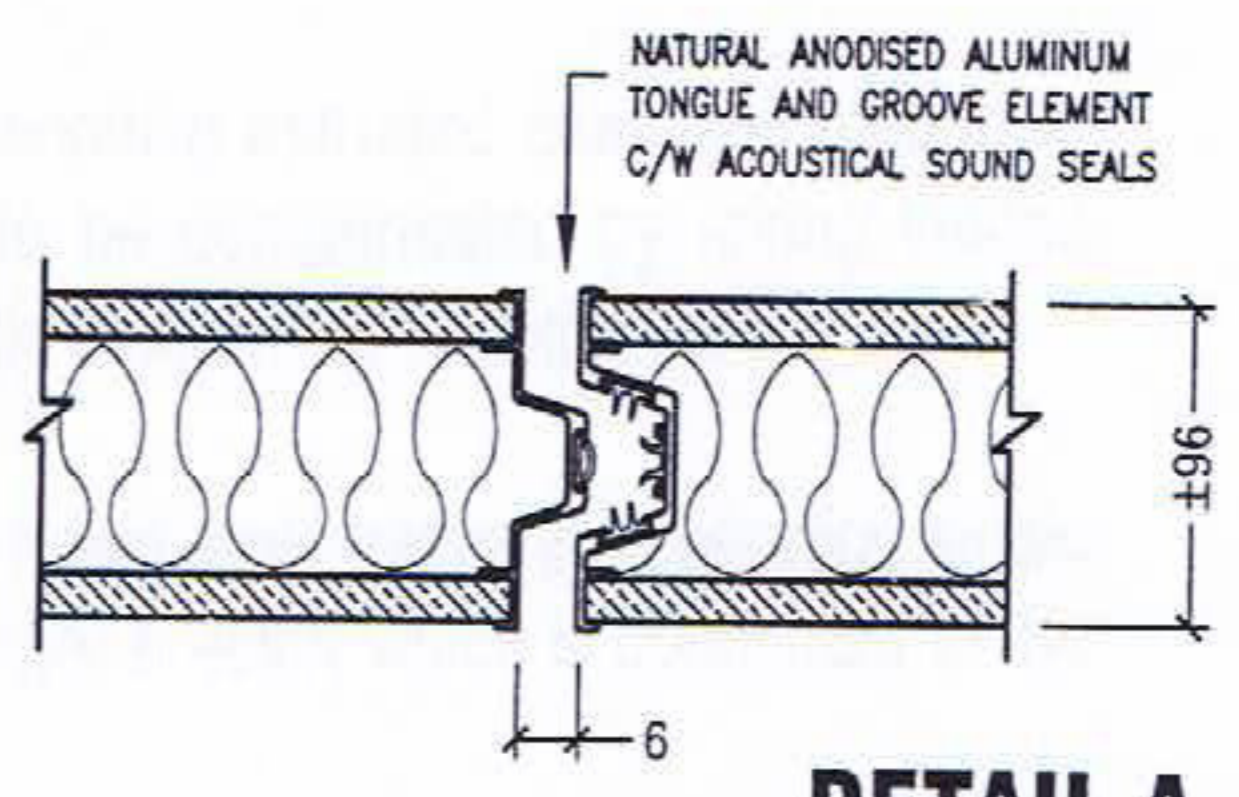
DETAIL A
